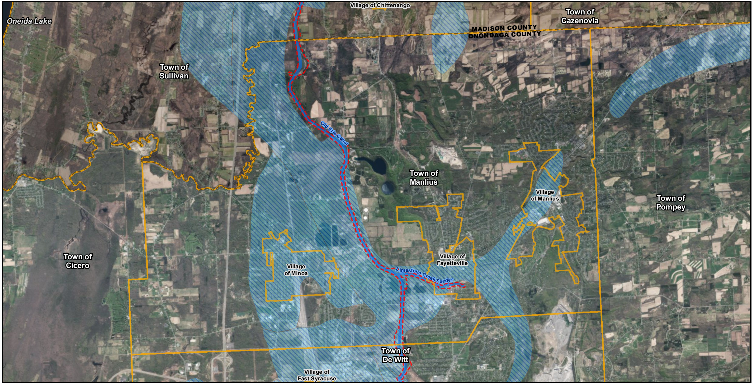
Figure 62F: Aquifers
